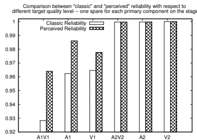
Figure 6: Comparison between \mathcal{R}(t) and \hat{\mathcal{R}}(t) .
