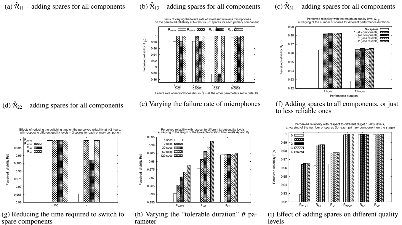
Figure 5: Perceived reliability \hat{\mathcal{R}}(t) for different stage configurations and with respect to different quality levels
